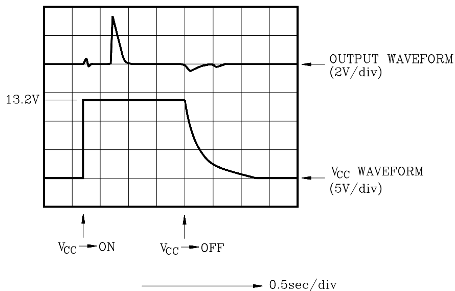
Fig. 5 BTL OPERATION
