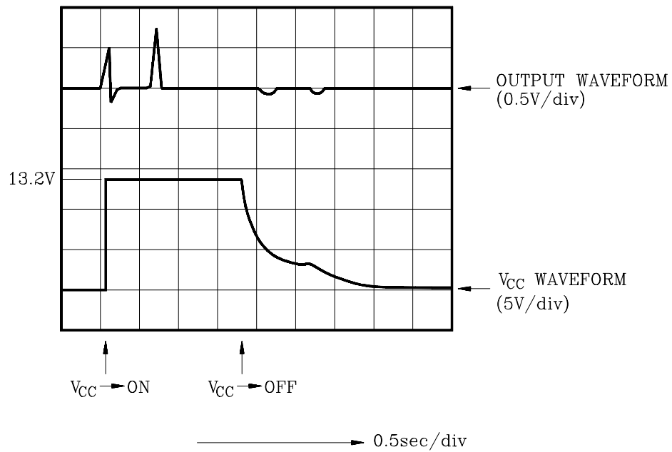
Fig. 6 DUAL OPERATION
